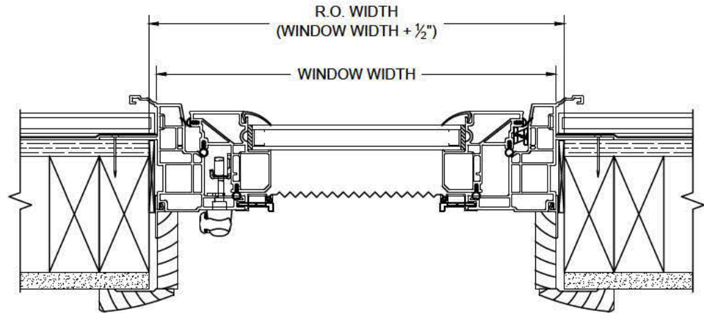
HORIZONTAL SECTION 2 x 4 Construction w/ Extension Jamb and Exterior Siding
