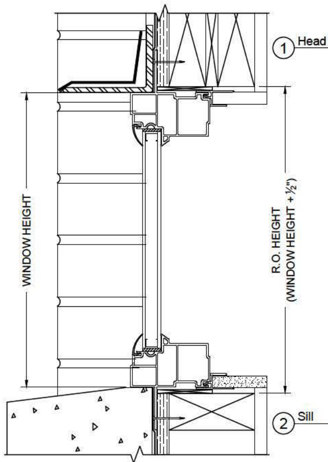
VERTICAL SECTION 2 x 4 Construction w/ Drywall Return and Face Brick
