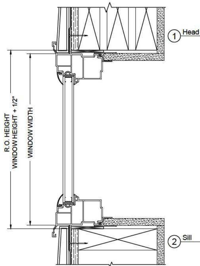
VERTICAL SECTION 2 x 6 Construction w/ Drywall Return and Exterior Siding
