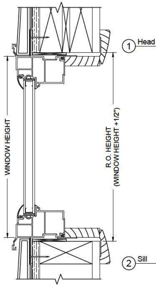
VERTICAL SECTION 2 x 4 Construction w/ Extension Jamb and Exterior Siding
