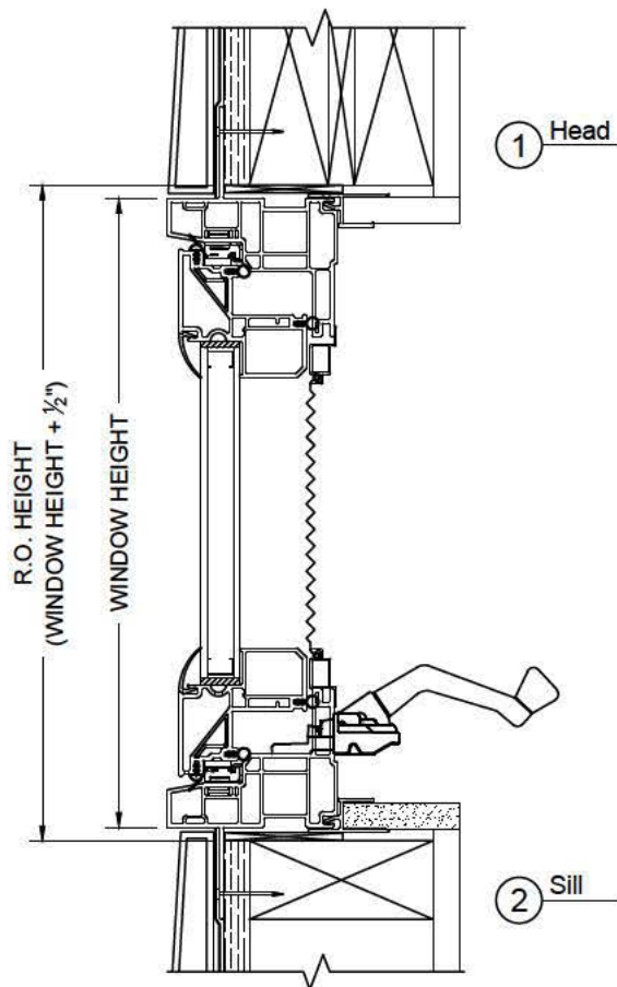
VERTICAL SECTION 2 x 4 Construction w/ Drywall Return and Exterior Siding
