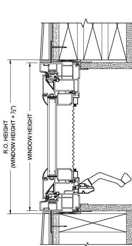
VERTICAL SECTION 2 x 6 Construction w/ Drywall Return and Exterior Siding
