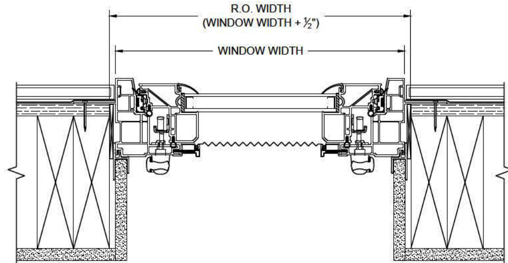
HORIZONTAL SECTION 2 x 6 Construction w/ Drywall Return and Exterior Siding
