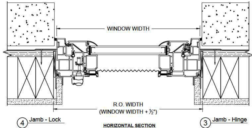
HORIZONTAL SECTION 2 x 4 Construction w/ Drywall Return and Face Brick
