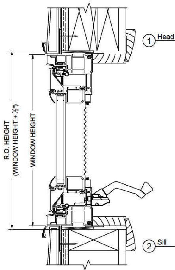
VERTICAL SECTION 2 x 4 Construction w/ Extension Jamb and Exterior Siding
