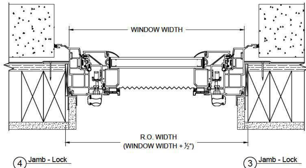
HORIZONTAL SECTION 2 x 4 Construction w/ Drywall Return and Face Brick
