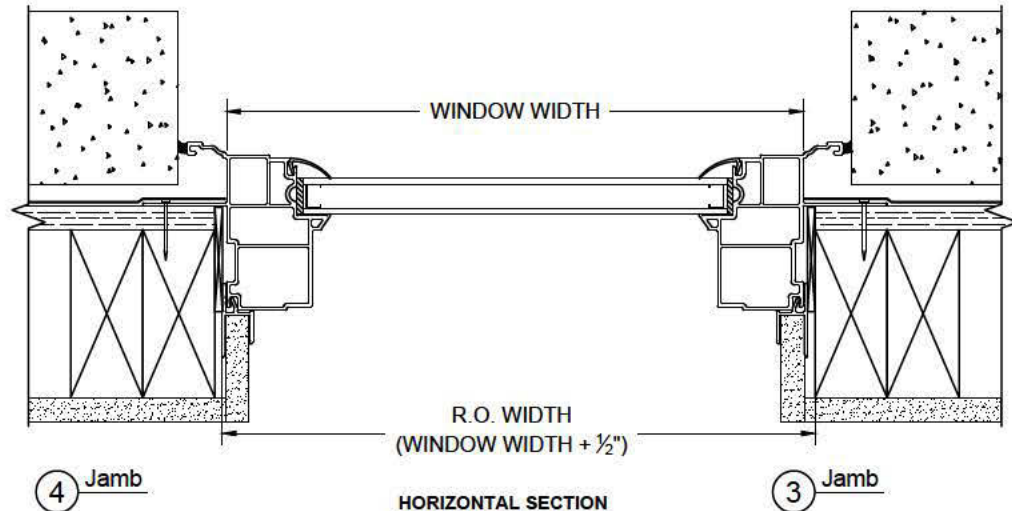
HORIZONTAL SECTION 2 x 4 Construction w/ Drywall Return and Face Brick
