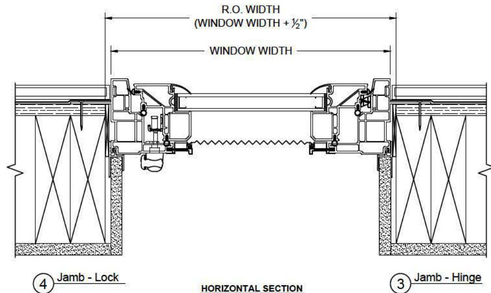
HORIZONTAL SECTION 2 x 6 Construction w/ Drywall Return and Exterior Siding
