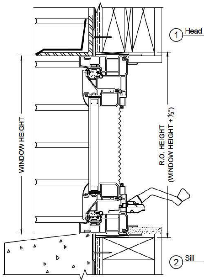
VERTICAL SECTION 2 x 4 Construction w/ Drywall Return and Face Brick
