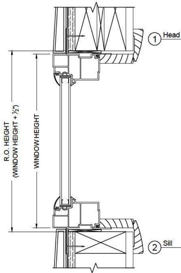
VERTICAL SECTION 2 x 4 Construction w/ Extension Jamb and Exterior Siding
