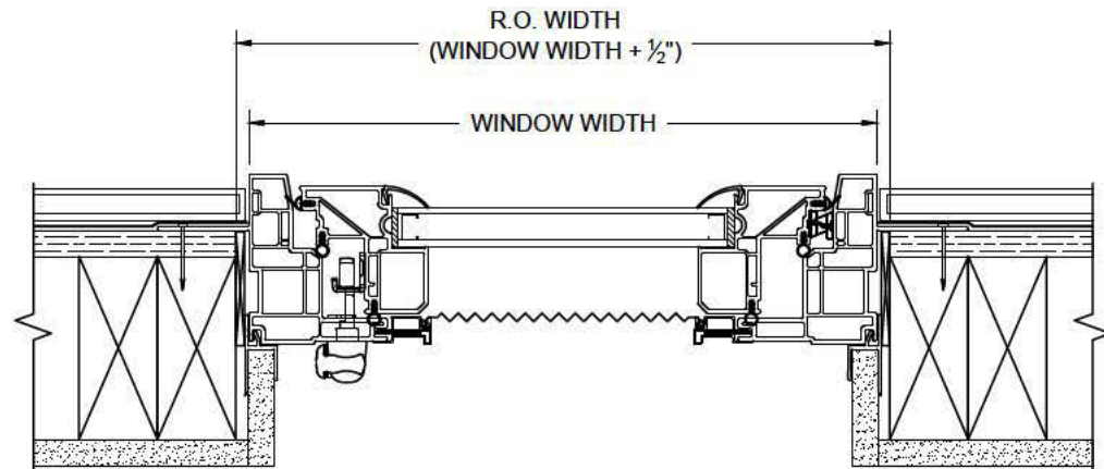
HORIZONTAL SECTION 2 x 4 Construction w/ Drywall Return and Exterior Siding
