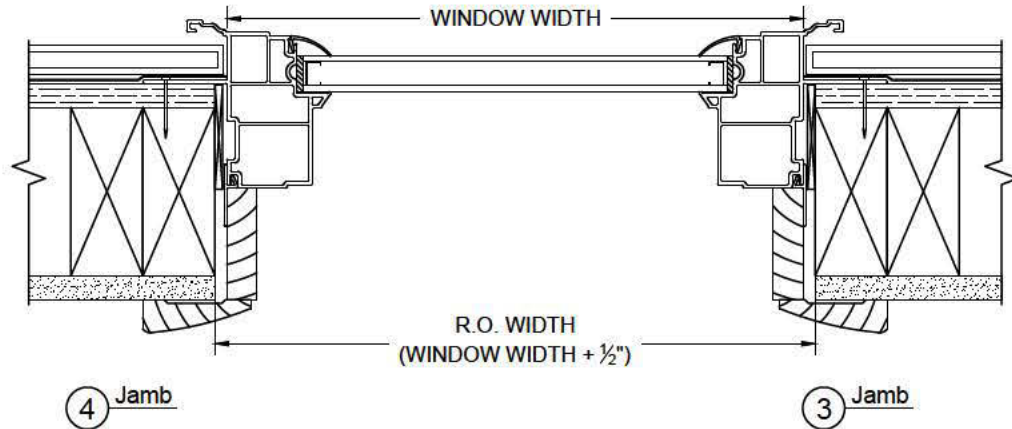
HORIZONTAL SECTION 2 x 4 Construction w/ Extension Jamb and Exterior Siding
