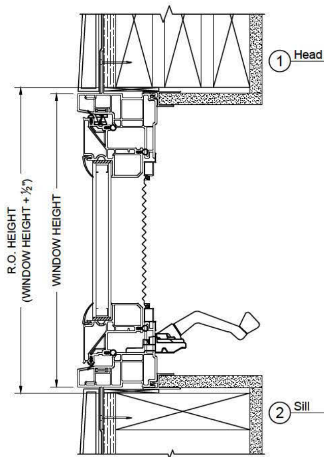
VERTICAL SECTION 2 x 6 Construction w/ Drywall Return and Exterior Siding
