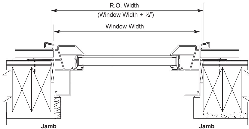
Horizontal Section 2 x 4 Frame Construction w/ Exterior Siding Scale: 3" = 1'0" (1:4)
