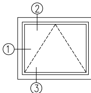
70RAW1 Replacement Awning Window Installation Elevation
