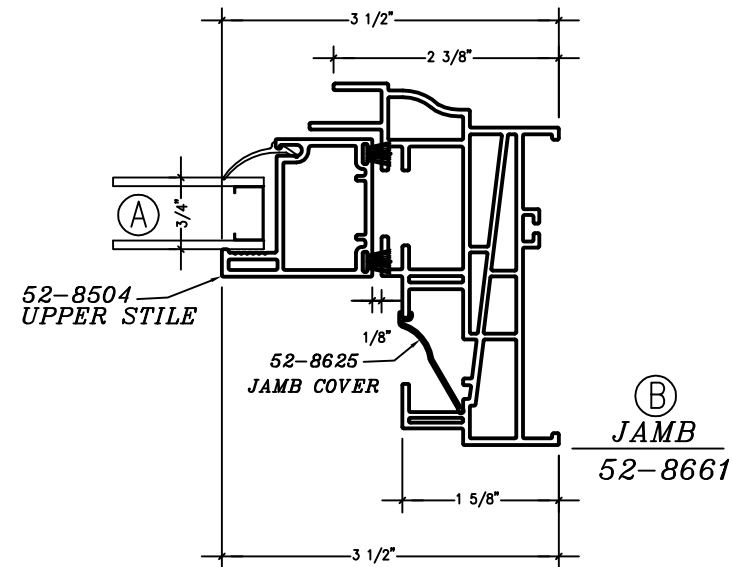
⑤ JAMB DETAIL THRU UPPER SASH
