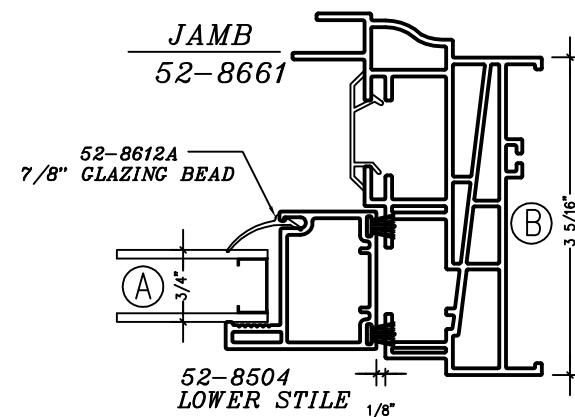
① JAMB DETAIL THRU LOWER SASH
