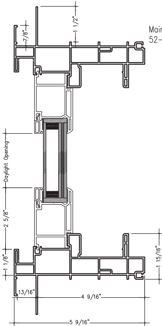
VERTICAL SECTION VIEW
