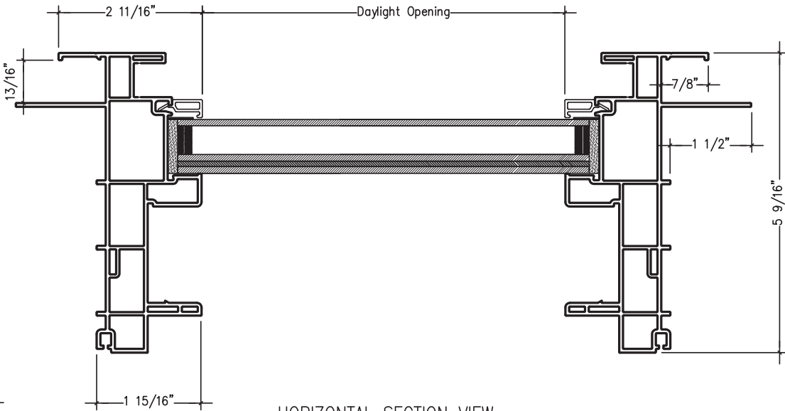
HORIZONTAL SECTION VIEW
