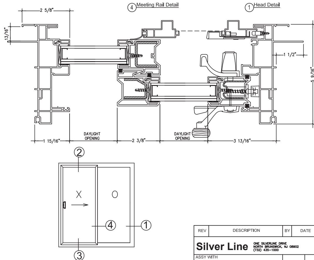
SERIES 5800 TWO PANEL PATIO DOOR
