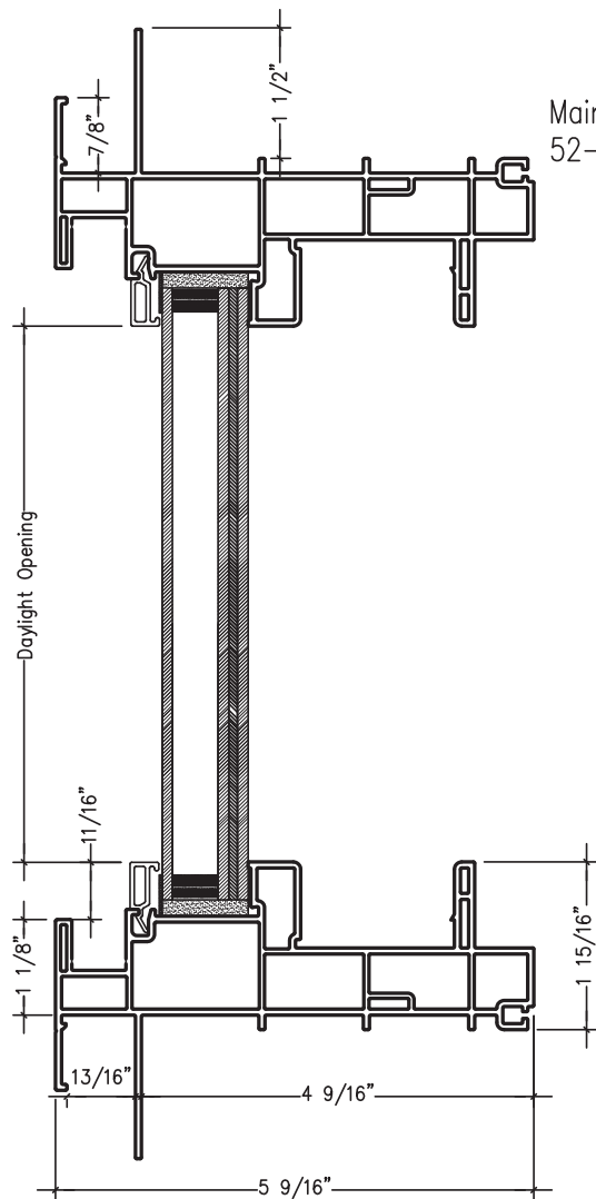
VERTICAL SECTION VIEW
